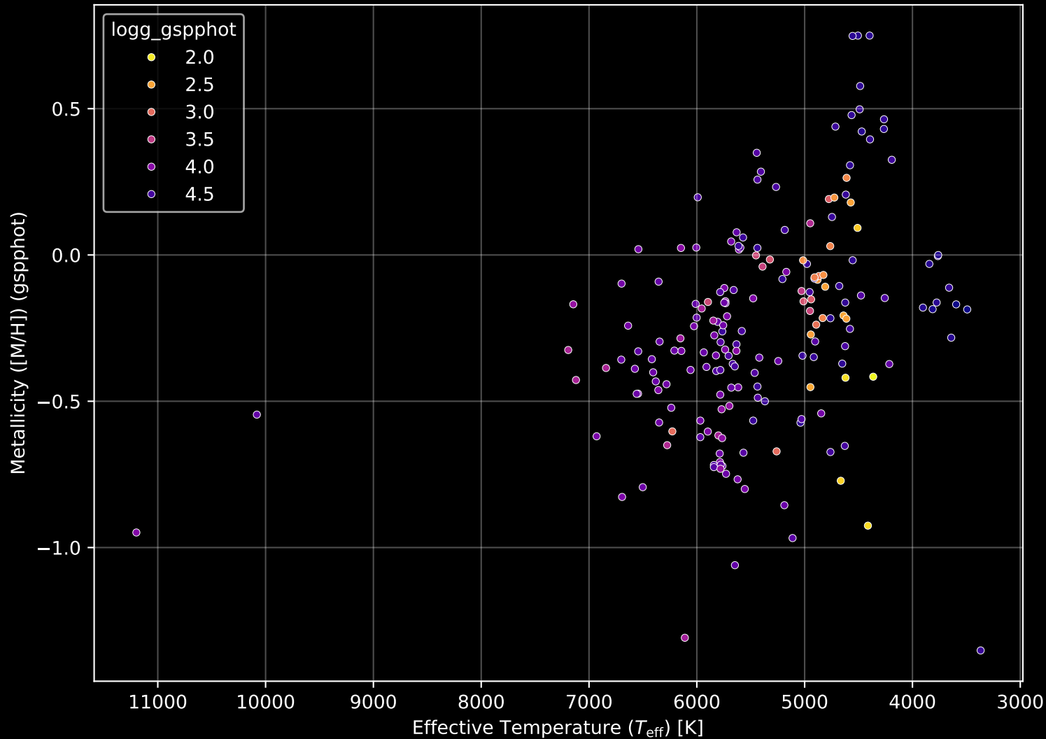
APOGEE DR17 Field: [197-39_MGA] Stellar Population Parameters (n= 190)
