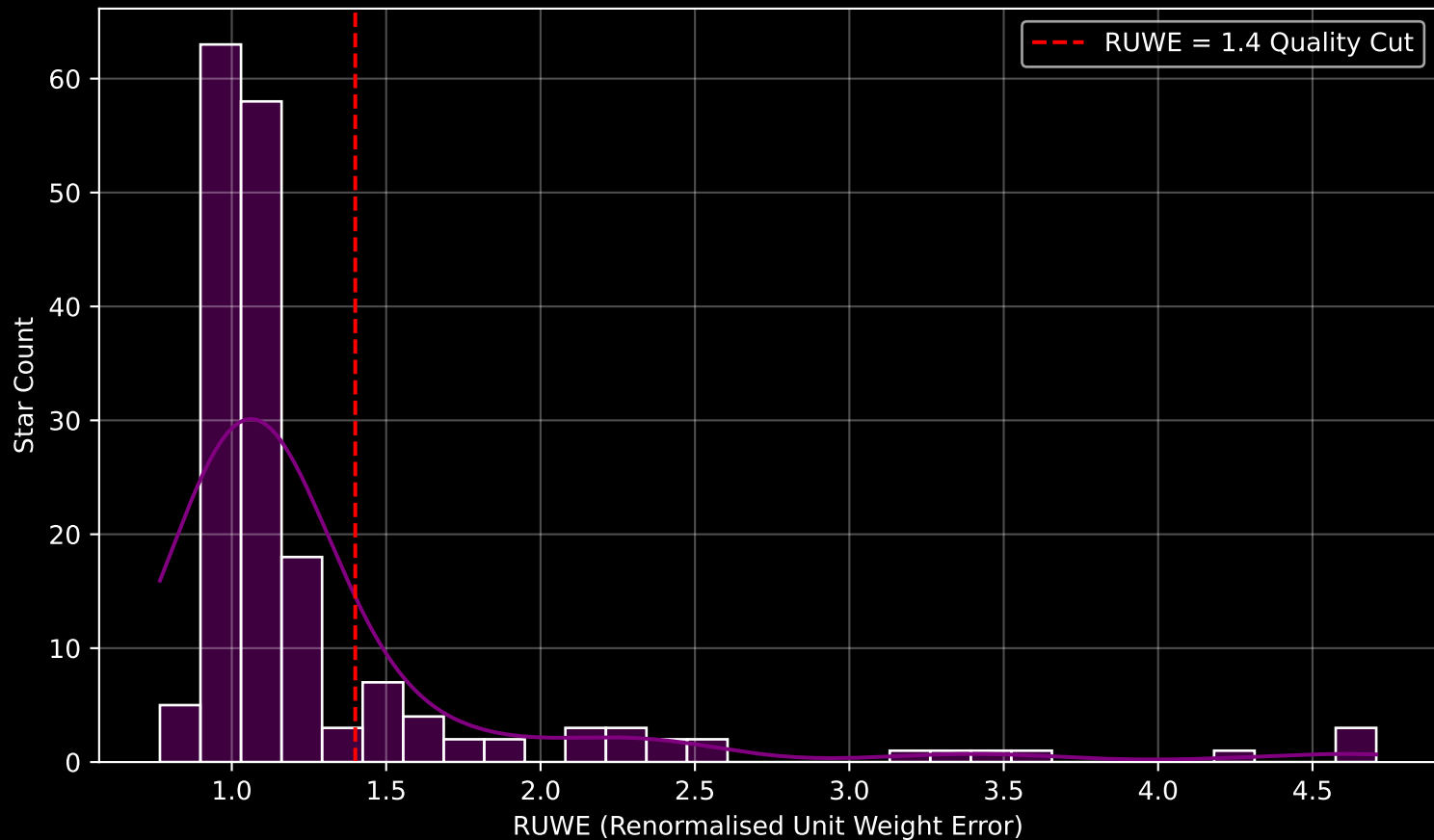
GAPOGEE DR17 Field [197-39_MGA] RUWE Distribution (n= 180)
