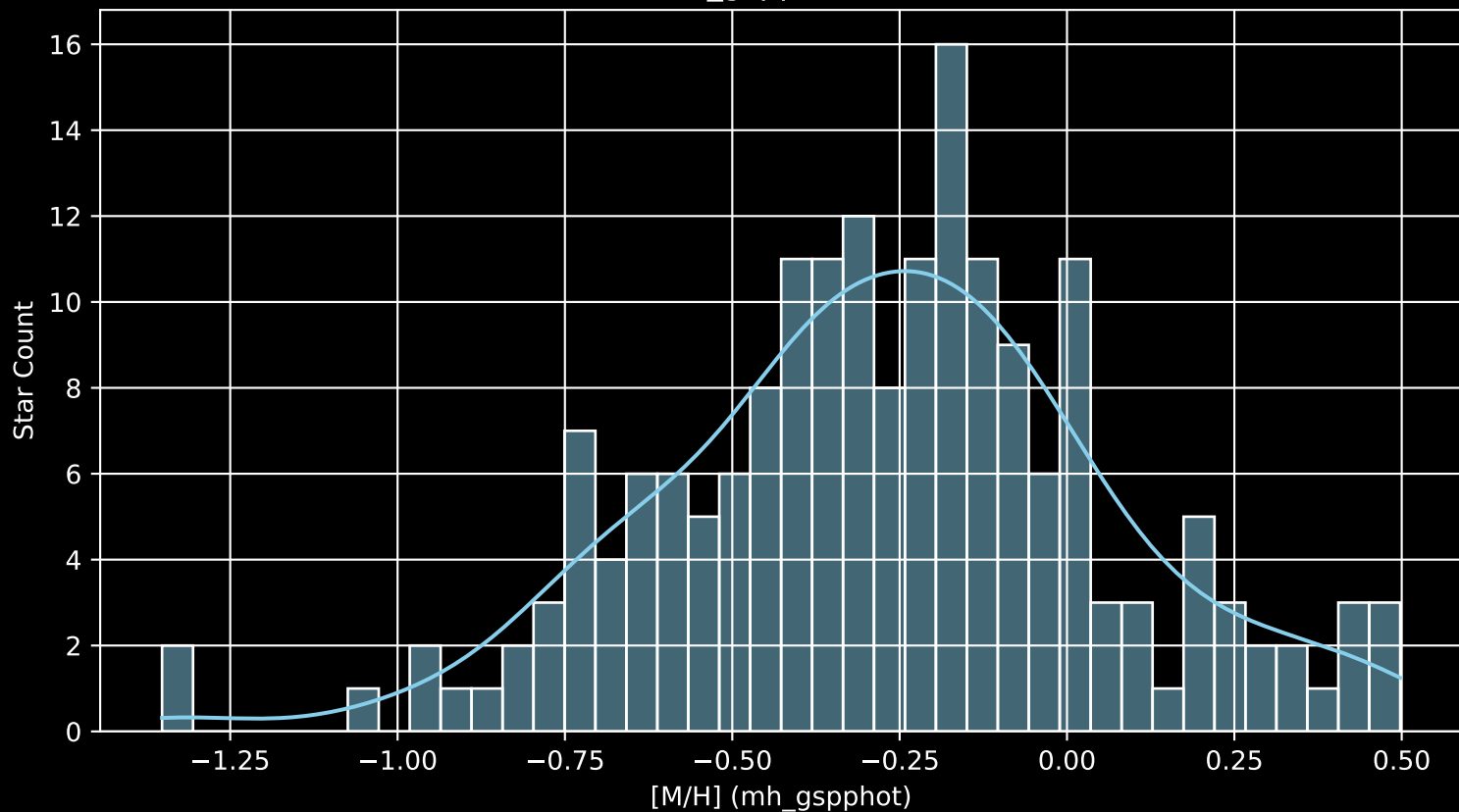
APOGEE DR17 Field: [197-39_MGA [M/H] (mh_gspphot) (n= 186)
