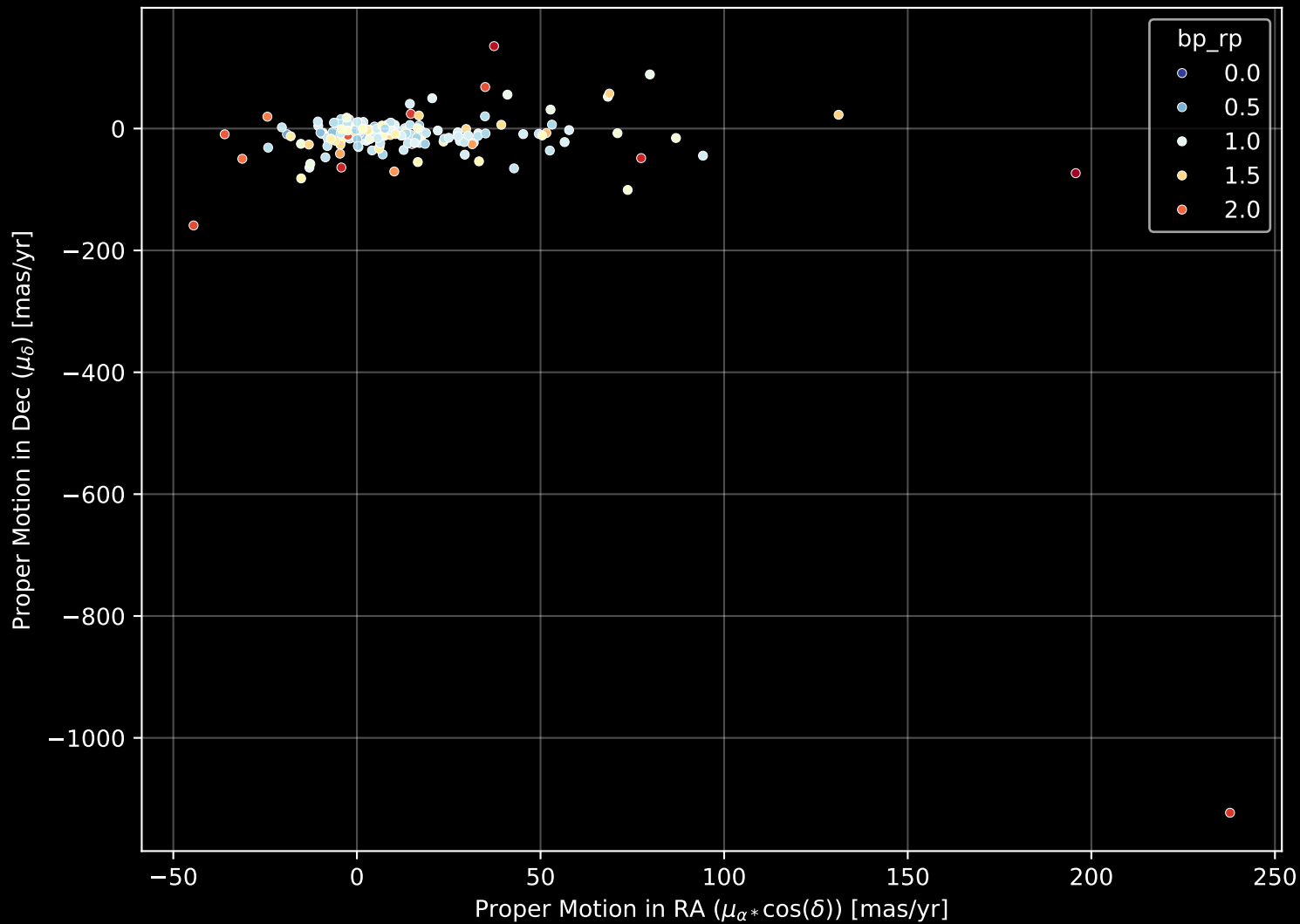
APOGEE DR17 Field: [197-39_MGA] Proper Motion Diagram (n= 190)
