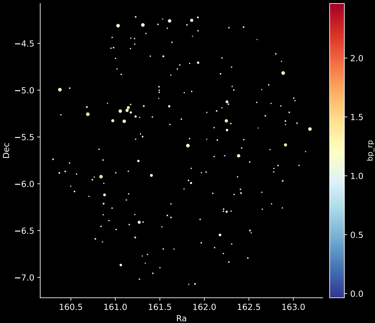
APOGEE DR17 Field: [197-39_MGA] Stars: 190
