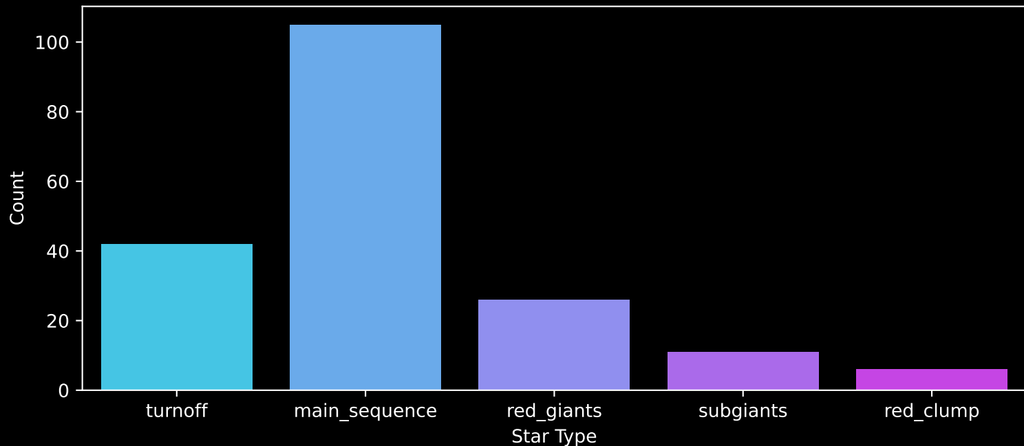
APOGEE DR17 Field: [197-39_MGA] Count plot of Star Type
