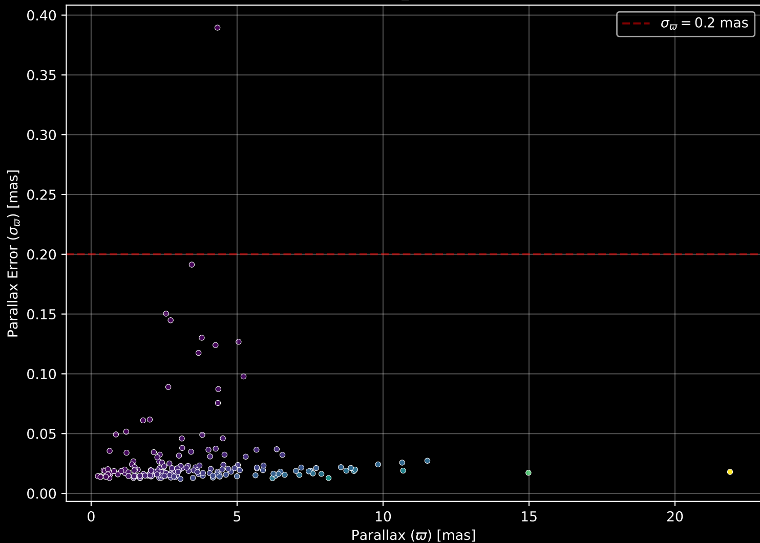
APOGEE DR17 Field: [197-39_MGA] Parallax Quality (n= 190)
